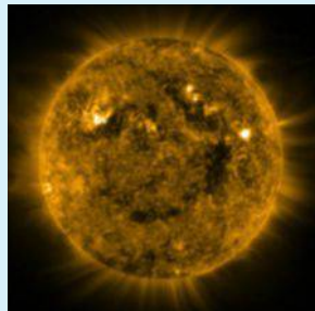
Solar Imaging
