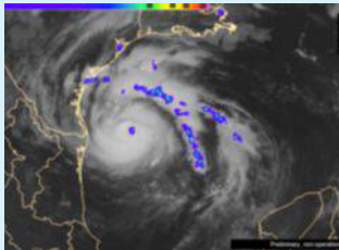
Lightning Mapping
